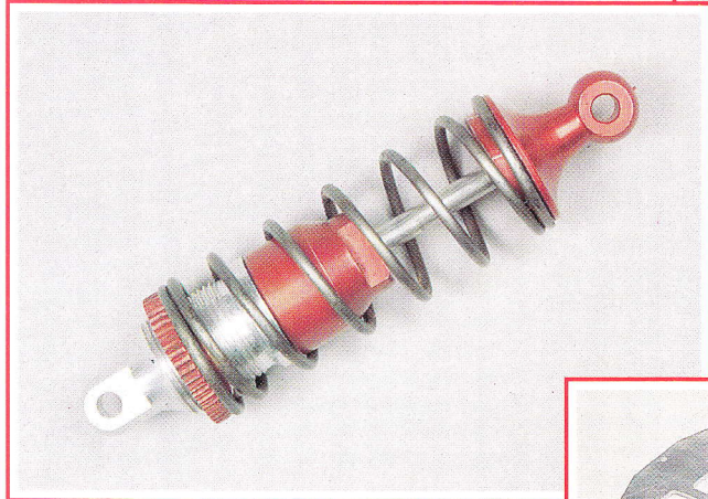
Art. 708230000 Anteriori - Front Art. 708240000 Posteriori - Rear Ammortizzatori a volume costante Permanent oil volume shock absorber
