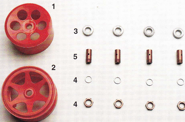
2 Art. 24371 Cerchi stretti - Narrow rims Schmale Felgen
